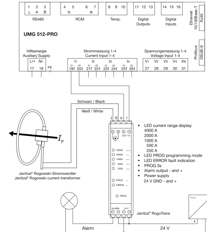
Example connections to a UMG 512-PRO
